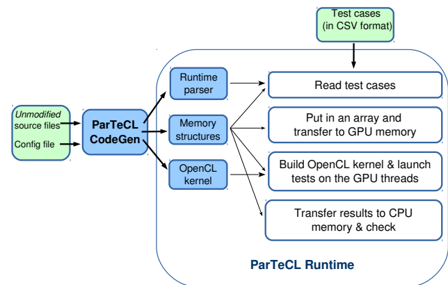
Figure 1: ParTeCL: automated test execution on the GPU.
