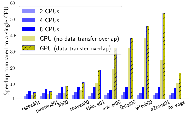
Figure 6: Speedup of GPU and multi-core CPUs over single CPU core.
