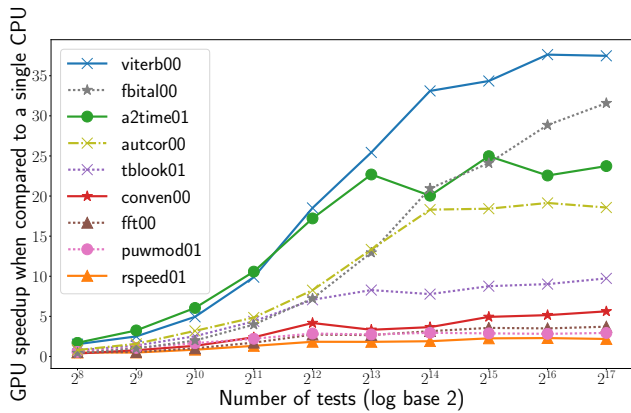
Figure 5: Speedup on the GPU vs single thread execution for 10 different test suite sizes. GPU data transfer and kernel execution not overlapped.
